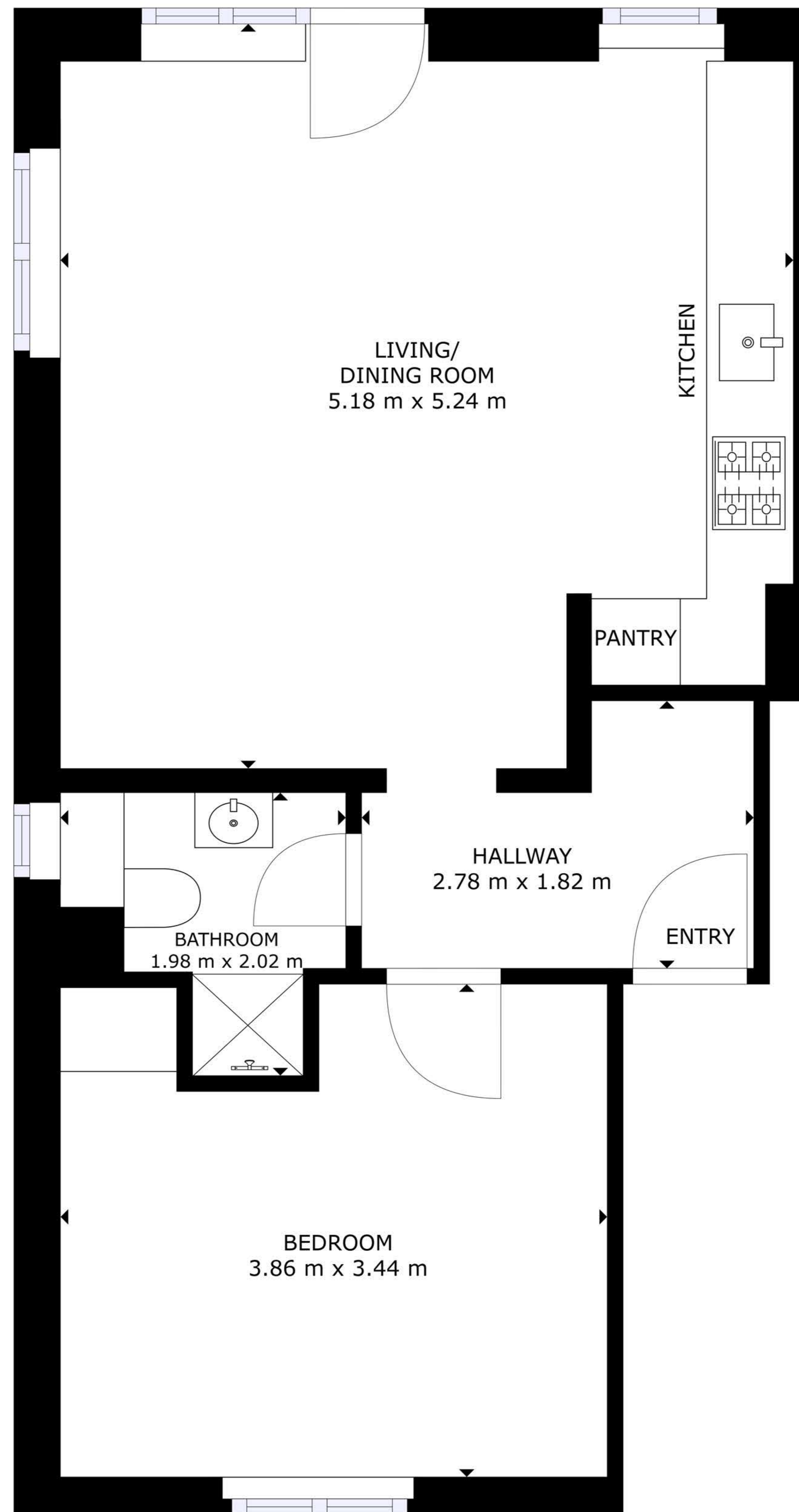
FLOOR PLAN
